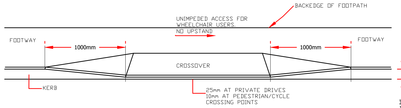
DISHED KERB DETAIL SCALE N.T.S
